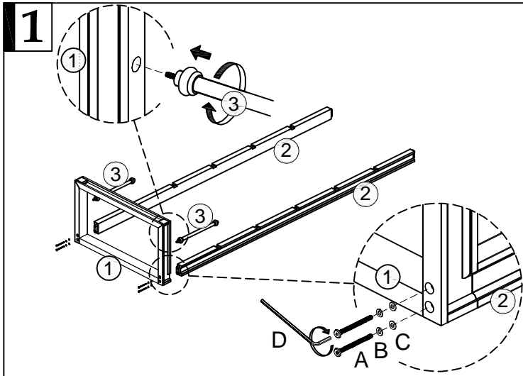
A Allen Bolt M6x70mm 20 pcs
