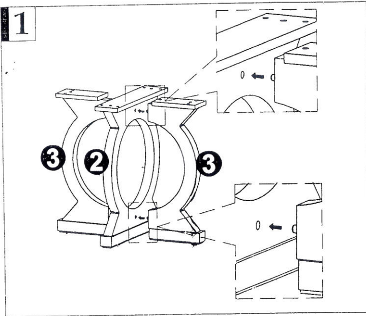
A Allen Bolt M6 x 25mm 8 pcs
